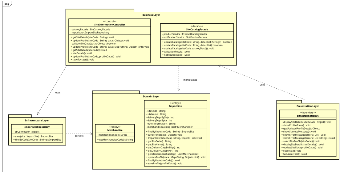
Hình 4.3: Package dependency diagram UC002 - ManageSiteInformation
