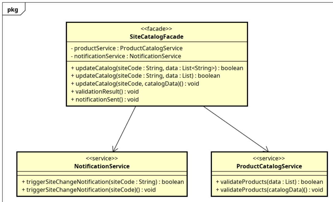
Hình 3.3: Class diagram subsystem UC002 - ManageSiteInformation
