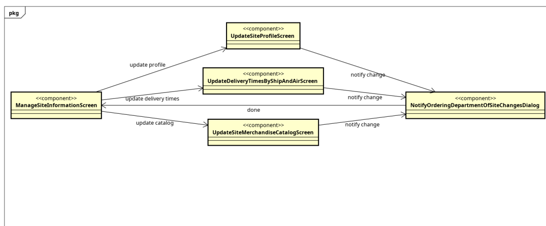
Hình 3.1: Screen transition diagram UC002 - ManageSiteInformation
