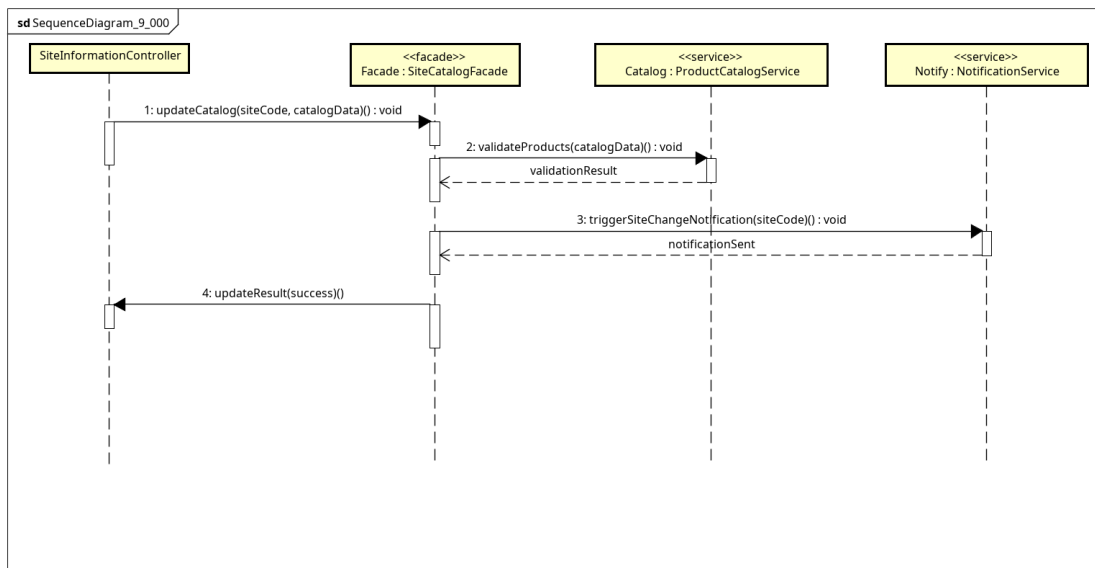
Hình 3.4: Sequence diagram subsystem UC002 - ManageSiteInformation
