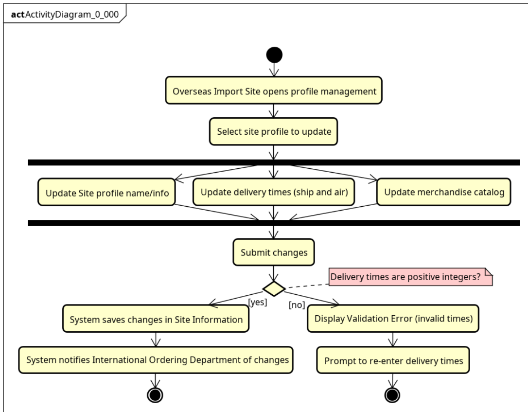
Hình 1.2: Activity diagram UC002 - ManageSiteInformation
